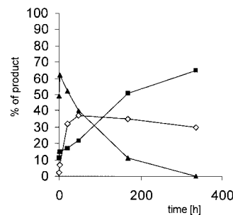
Figure 3. The time course for the formation of the phosphorus products in the reaction of 1a with LR (transformations of the AnsPSO species): \blacktriangle , adduct 2a ; \diamond , pyrothiophosphonate 3 ; \blacksquare , thiophosphonic acid 4 .
