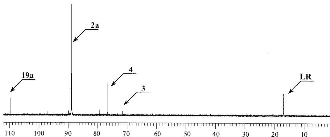
Figure 2. ^{31}\text{P} NMR spectrum of the crude reaction mixture obtained 2 min after LR was added to 1a at room temperature.
