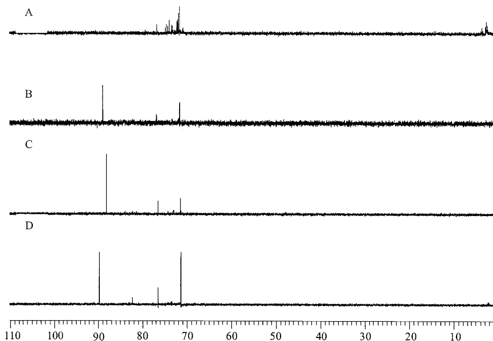
Figure 1. 31 P NMR spectra of the reaction mixtures (THF, room temp., 1 h) formed from LR and A) N -isopropylbenzamide, B) 1a (Ar = Ph), C) 1b (Ar = 4-MeOC 6 H 4 ), and D) 1c (Ar = 4-NO 2 C 6 H 4 ).
